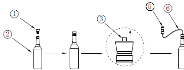
① Vacuum plug ② Wine bottle A ③ Valve B ⑤ Easy connector C ⑥ Connecting pipe D
